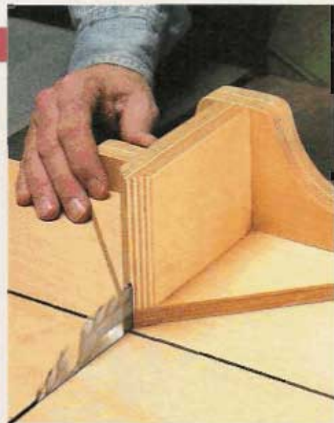
▲ Cutting a Kerf in the Sled. Once the sled is complete, you'll need to cut a kerf. To do this, raise the blade about 1 1/2". Next, push the sled through the blade (left) and complete the kerf by sliding the sled until the blade is "buried" half way into the blade housing (right).
