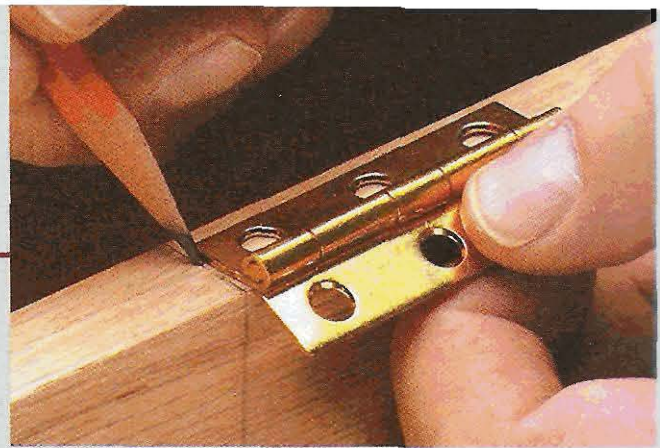
▲ Lay Out Location. The first step in routing a mortise for a hinge is to lay out the location of the hinge along the edge of the workpiece.
