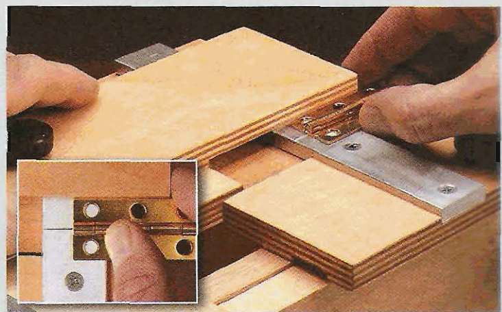
2 Here again, you can use the hinge to set the width of the mortise. A typical installation is to adjust the back stop until the centerline of the knuckle lines up with the scribe mark (see inset).
