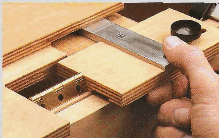
1 To set the length of the mortise, you can use the hinge to position the two parts of the base. Just be sure the inside edge of each base contacts the leaves of the hinge.
