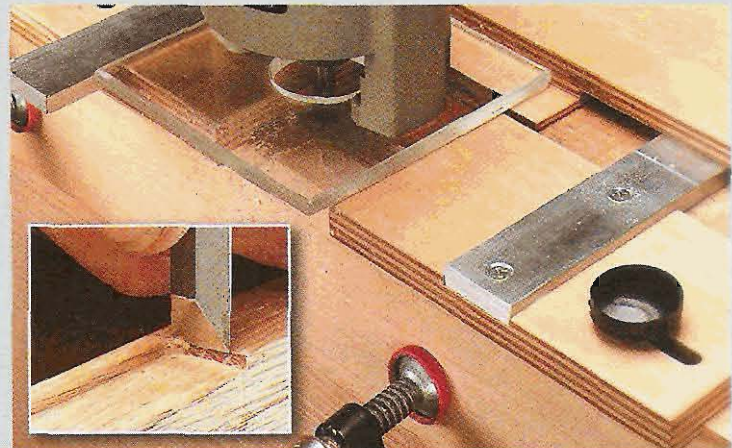
4 To remove most of the waste, rout clockwise around the inside edges of the aluminum guides and back stop. Then using the jig as a guide, square up the corners with a sharp chisel (inset).
