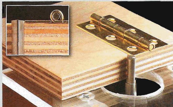
3 The depth of a hinge mortise often depends on the project design. In the photos above, a 1/2" spacer simulates the base of the jig while setting the bit to match the depth of the hinge leaf.
