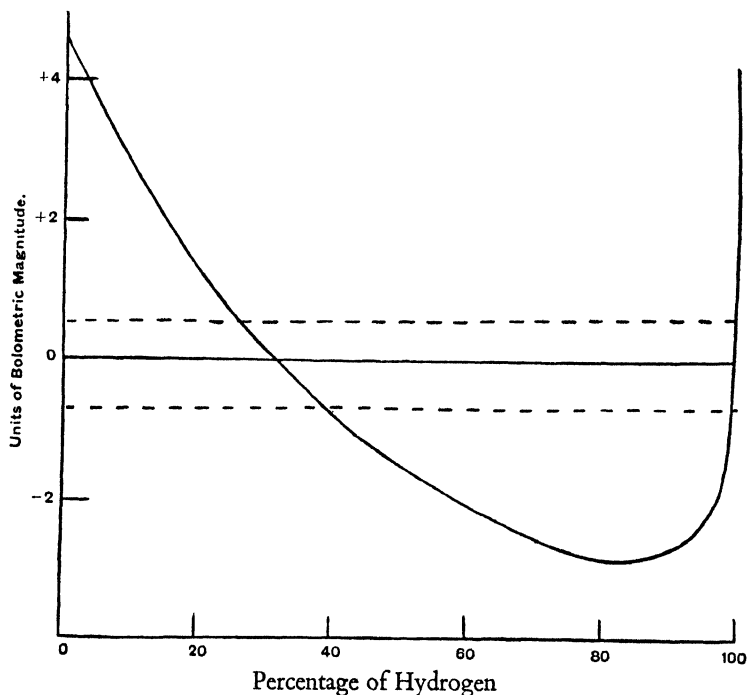
Theoretical Constitution of the Sun
